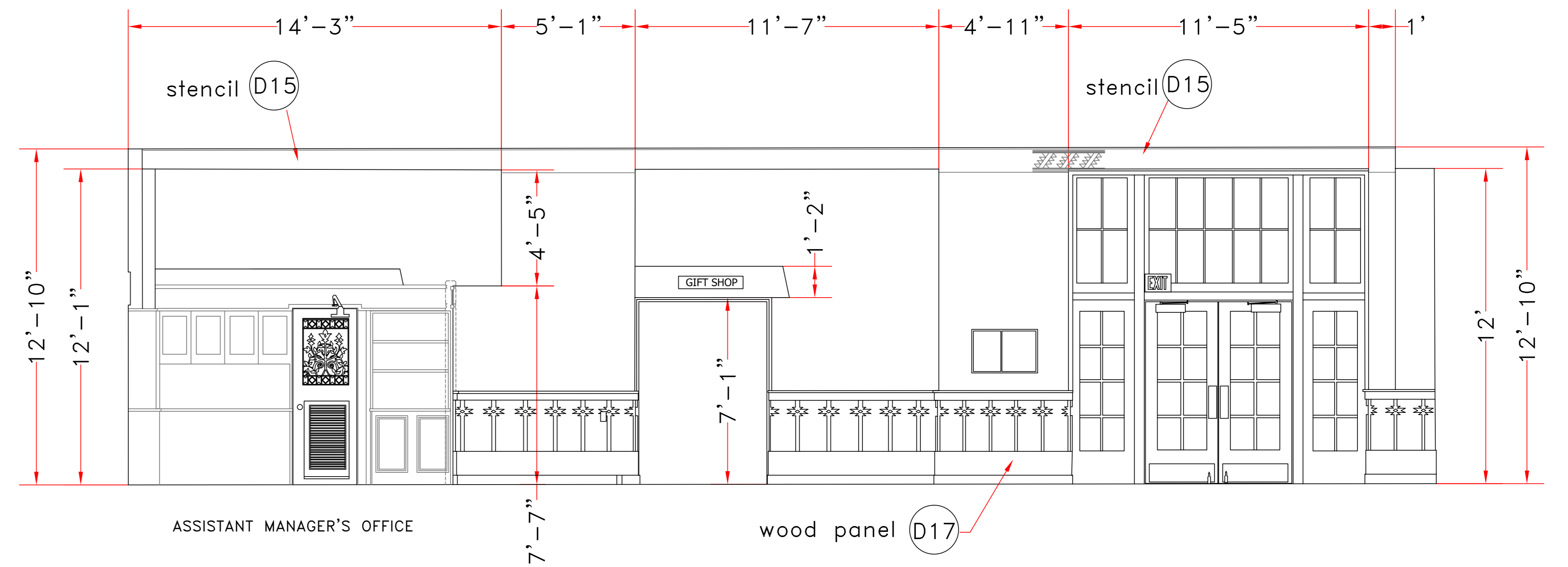
NORTH ELEVATION 2
