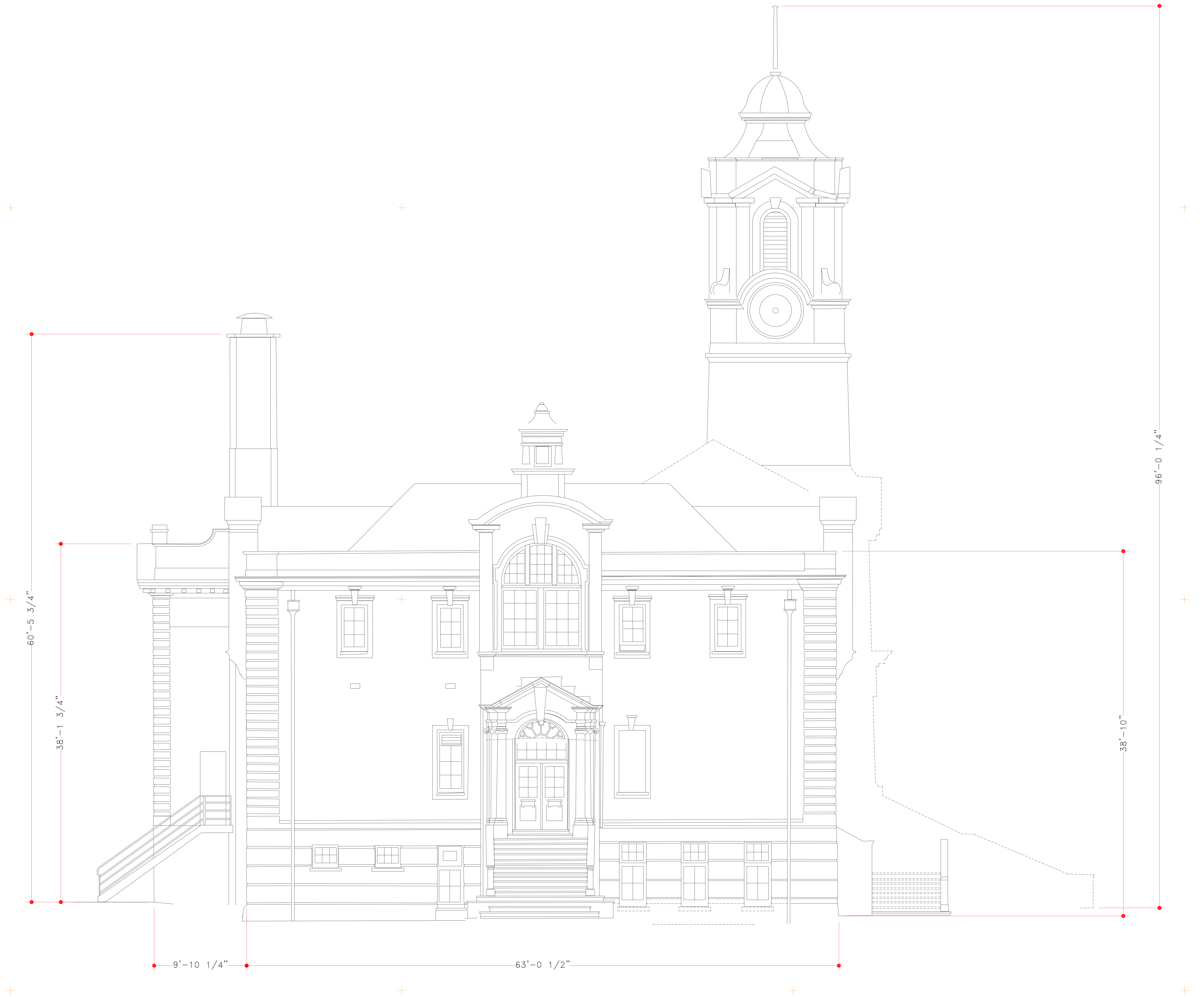
CAMOSUN YOUNG BUILDING – WEST ELEVATION
