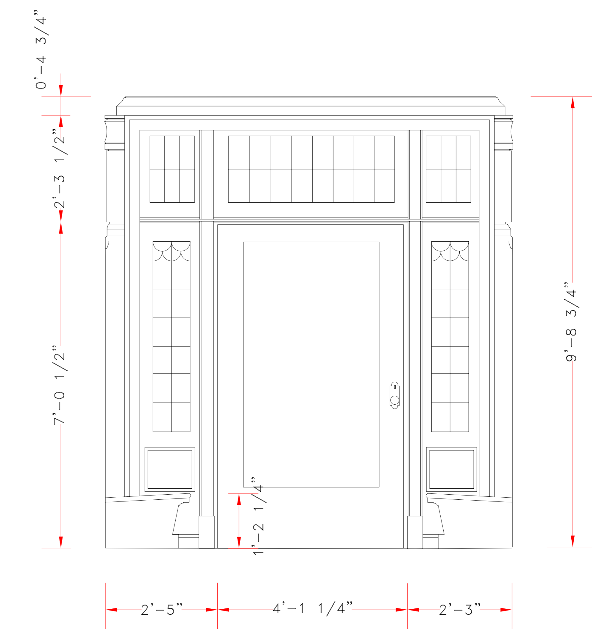
WEST ELEVATION – VESTIBULE
