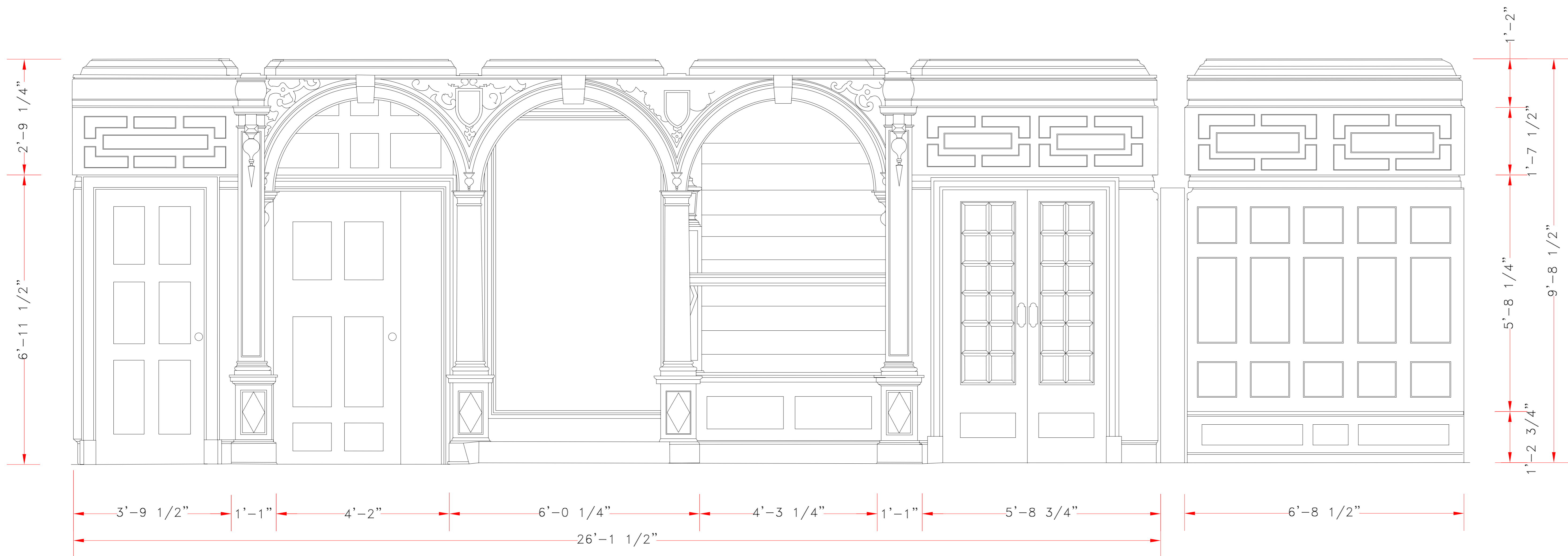
SOUTH ELEVATION – FOYER
