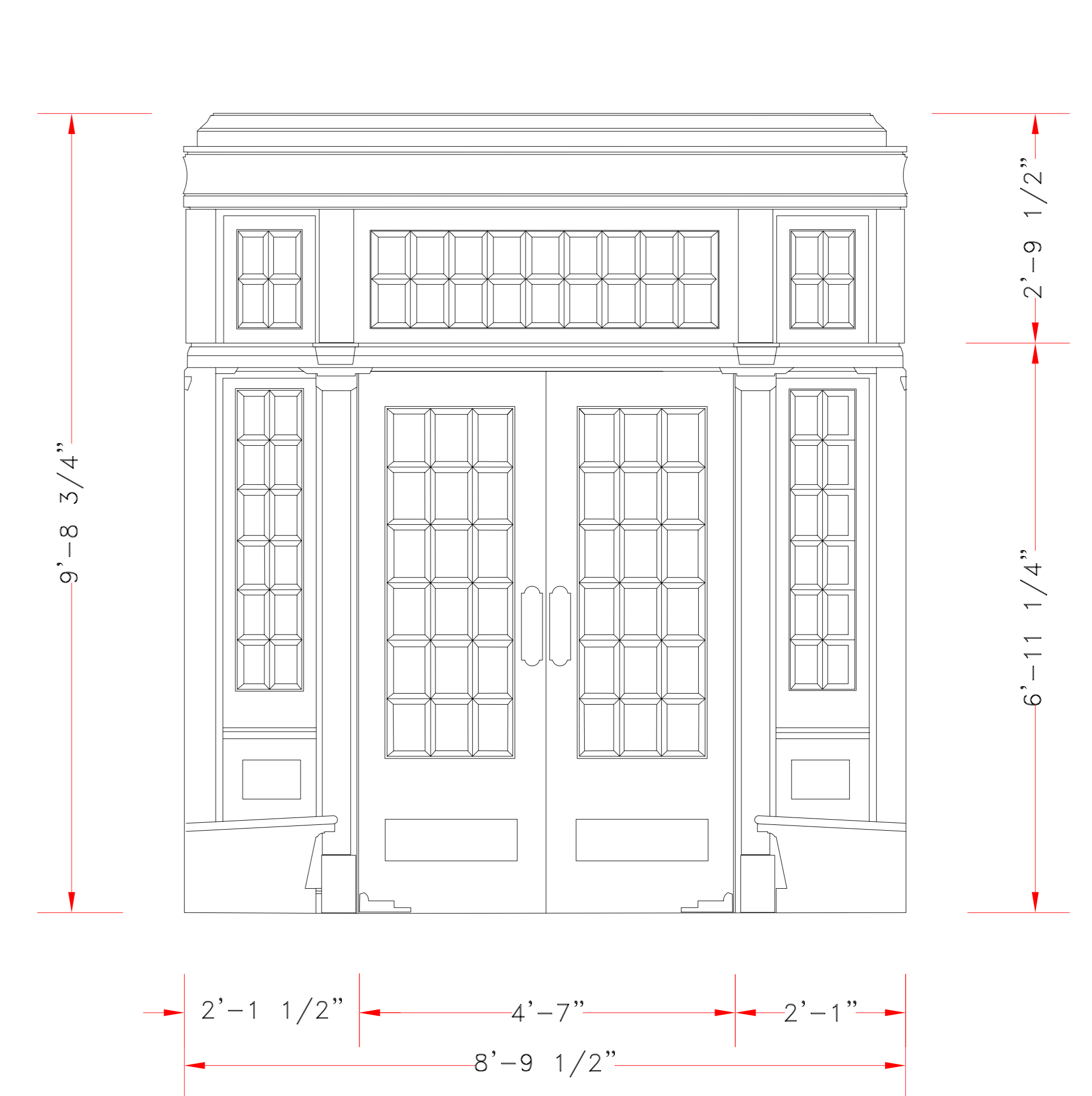
EAST ELEVATION – VESTIBULE
