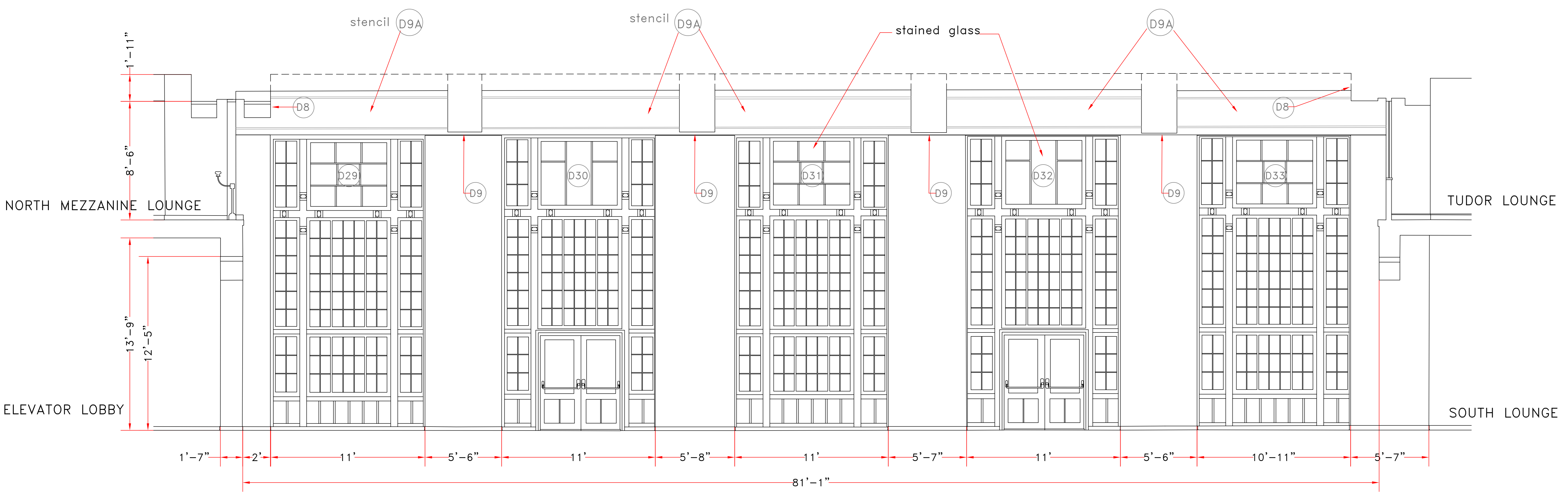
EAST ELEVATION
