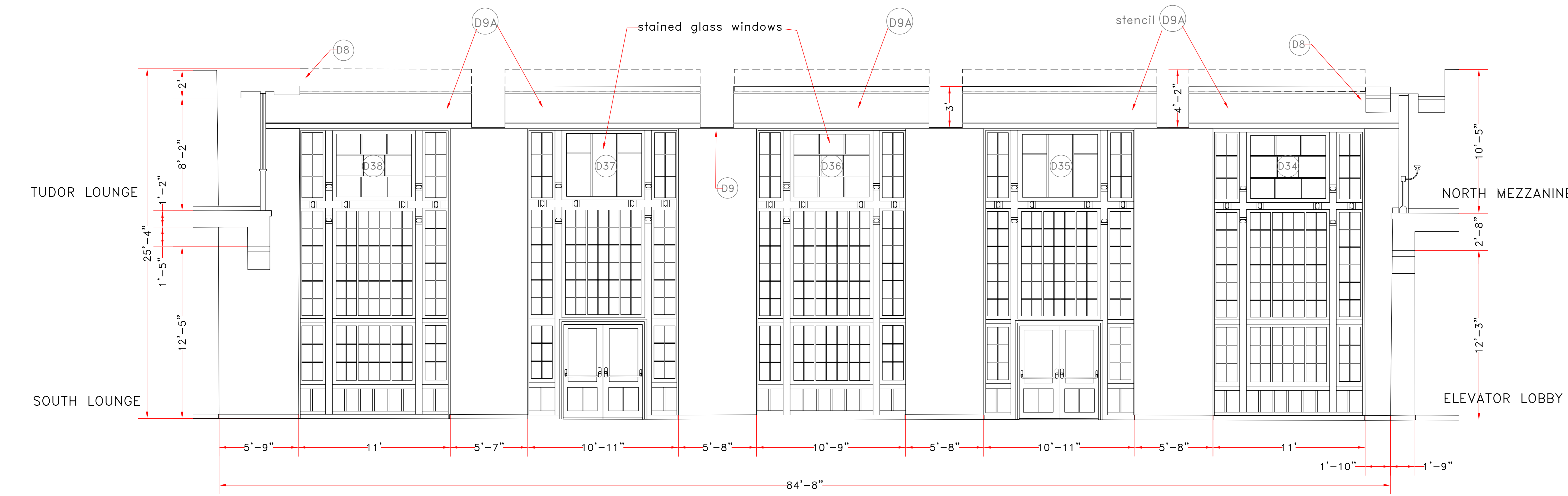
WEST ELEVATION
